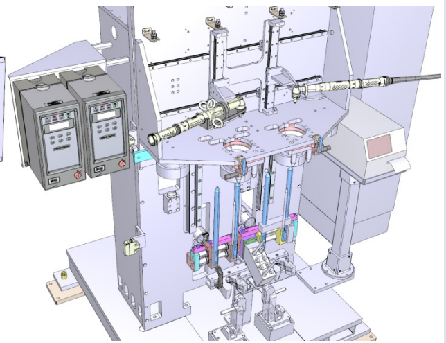
Abb. 2: Detail - Federbeinmontage
